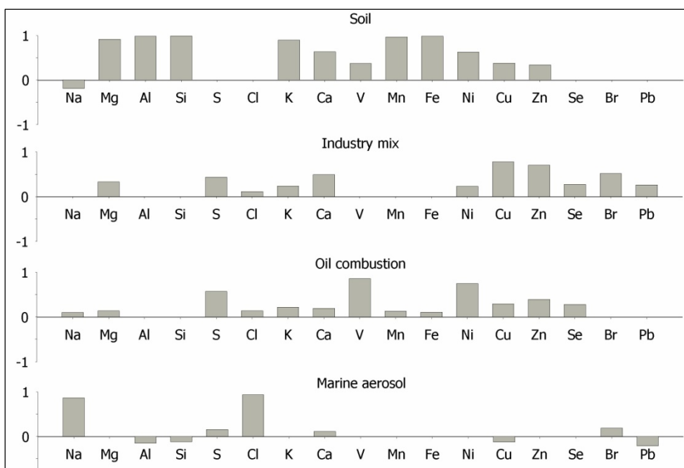
Figure 3. Varimax rotated factor loadings for chemical species of PM 10 combined from seven sites.
