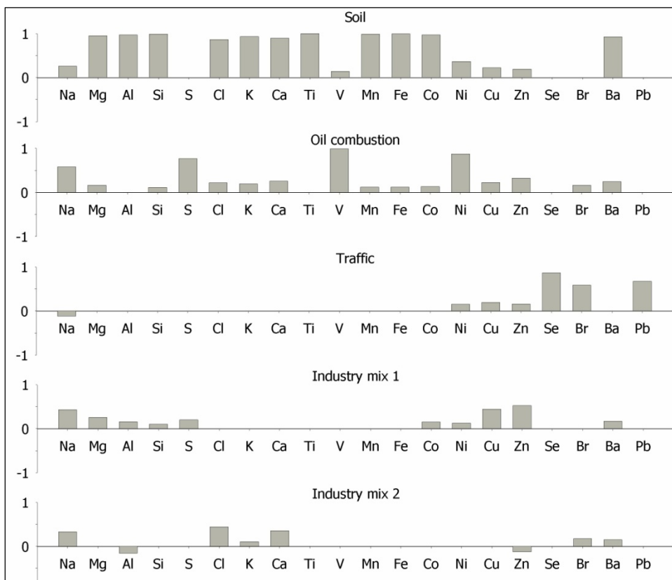
Figure 2. Varimax rotated factor loadings for chemical species of PM 2.5 combined from seven sites.
