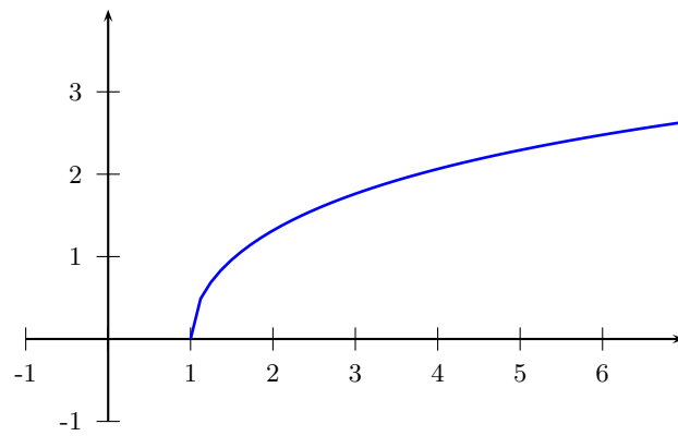
The graph of y = \cosh^{-1} x
