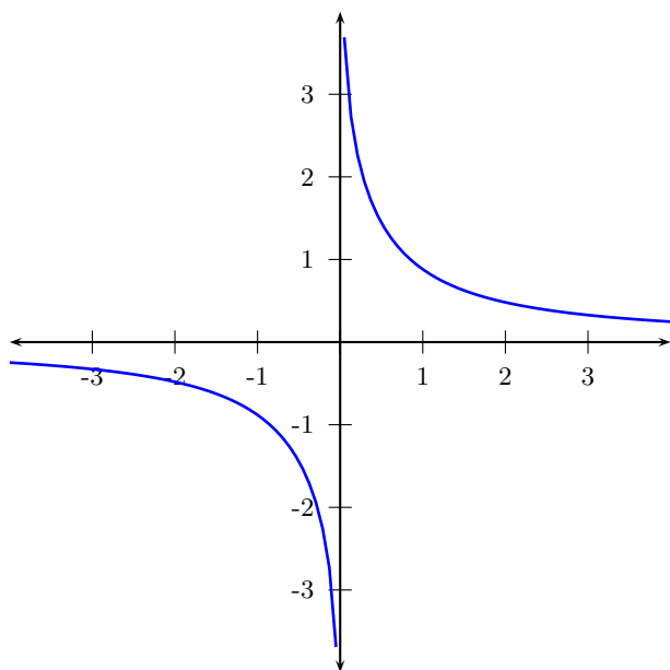
The graph of y = \operatorname{csch}^{-1}x
