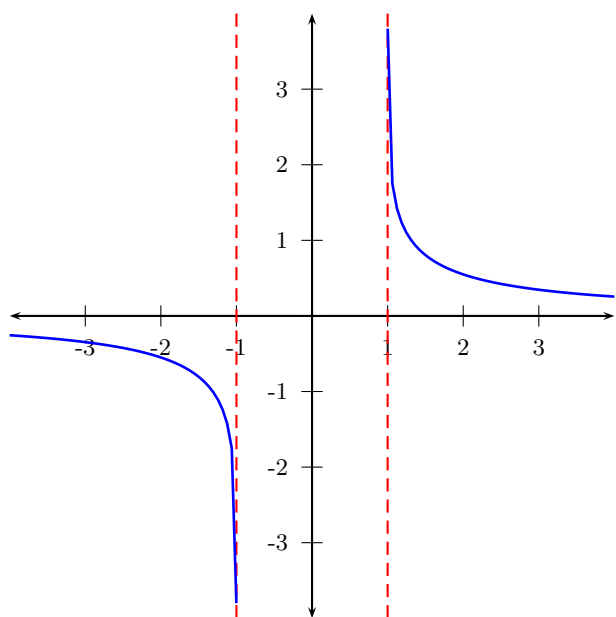
The graph of y = \operatorname{coth}^{-1}x
