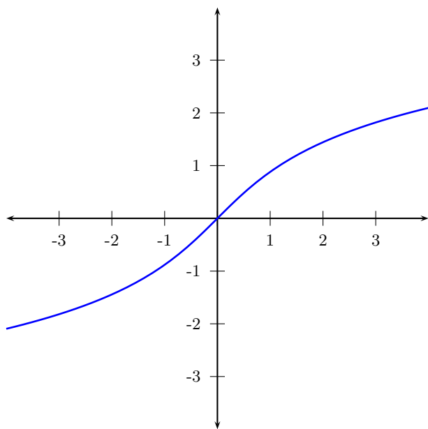
The graph of y = \sinh^{-1} x
