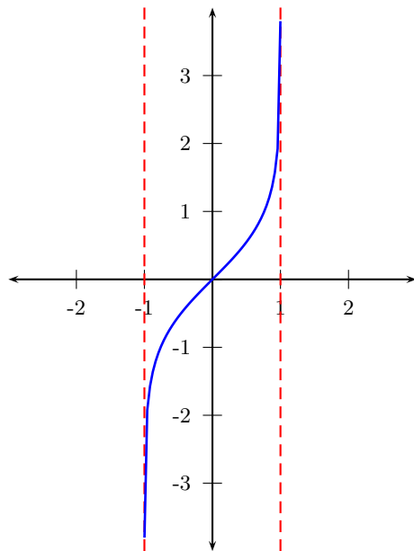
The graph of y = \tanh^{-1} x
